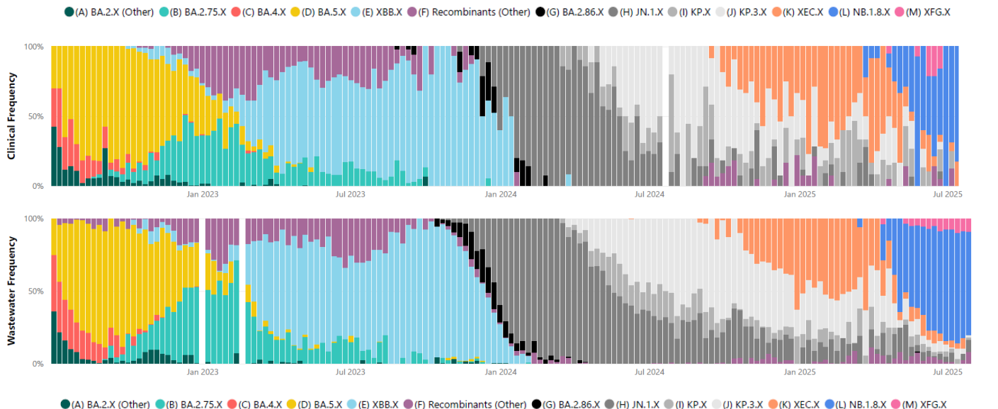
Figure 18. Distribution of SARS-CoV-2 variants in clinical samples (top) and metropolitan wastewater catchments (bottom), 03 July 2022 to 20 July 2025.
