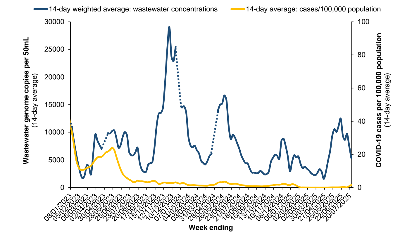
Figure 17. SARS-CoV-2 concentration in wastewater and COVID-19 notification rate, Perth metropolitan area, WA, 2023 to 25 July 2025.
