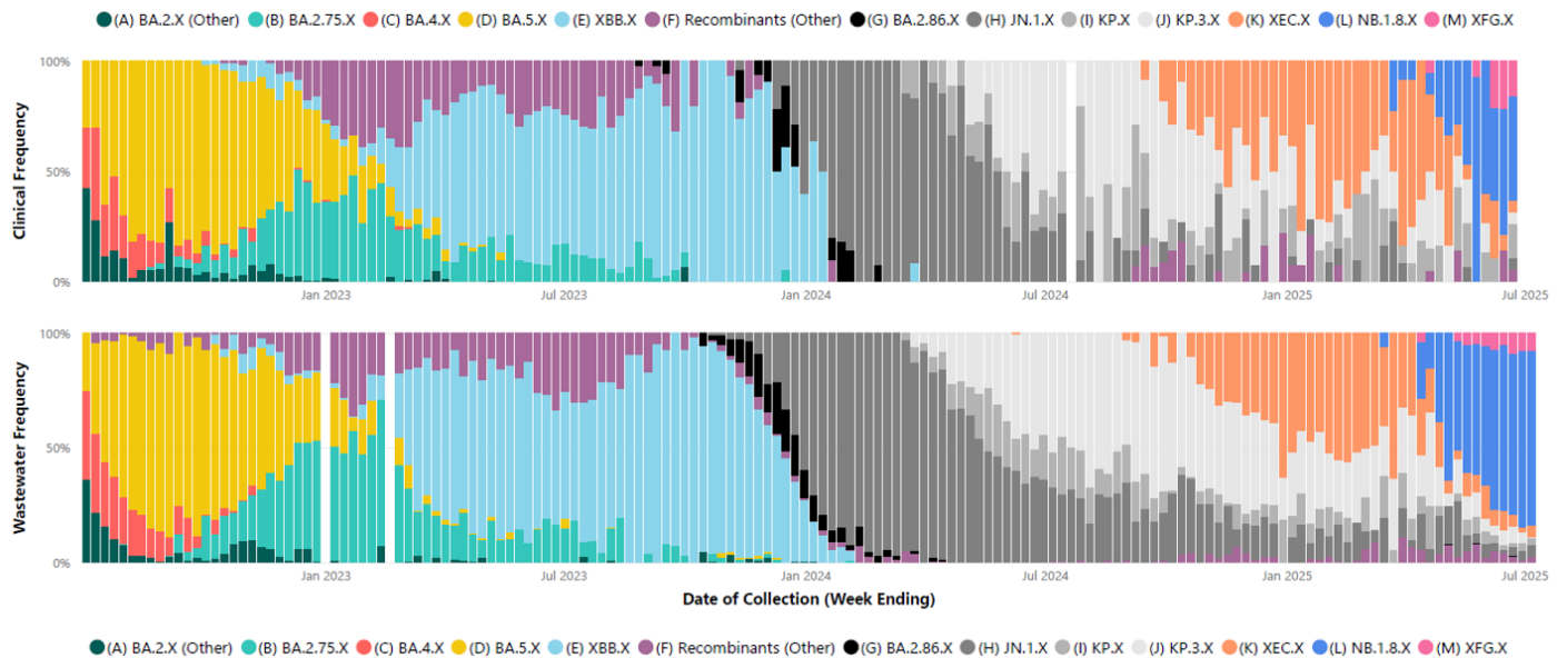
Figure 18. Distribution of SARS-CoV-2 variants in clinical samples (top) and metropolitan wastewater catchments (bottom), 03 July 2022 to 06 July 2025.
