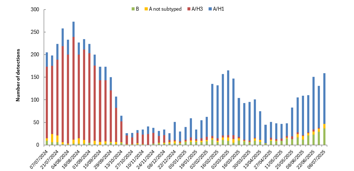
Figure 9. Number of PCR positive influenza detections at PathWest by type, subtype and week, WA, 2024 to 2025 YTD
