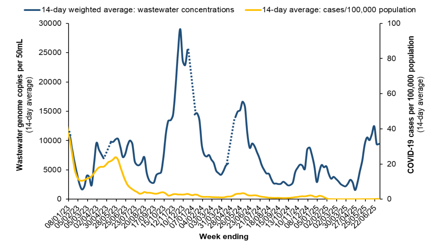
Figure 17. SARS-CoV-2 concentration in wastewater and COVID-19 notification rate, Perth metropolitan area, WA, 2023 to 04 July 2025.
