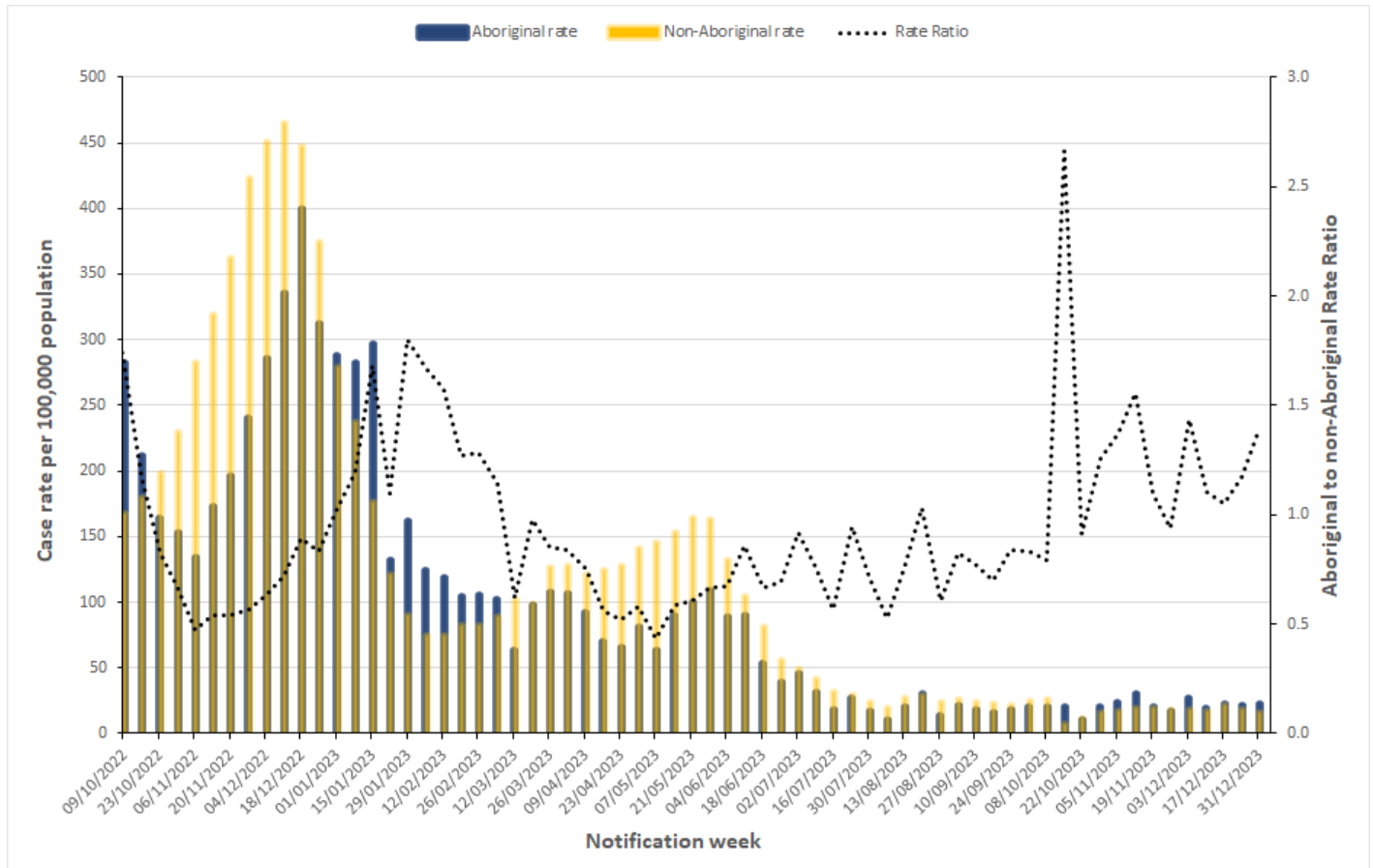
Figure 5. COVID-19 case rates per 100,000 population and rate ratio by Aboriginal status and notification week, Western Australia, 09 October 2022 to 31 December 2023.
